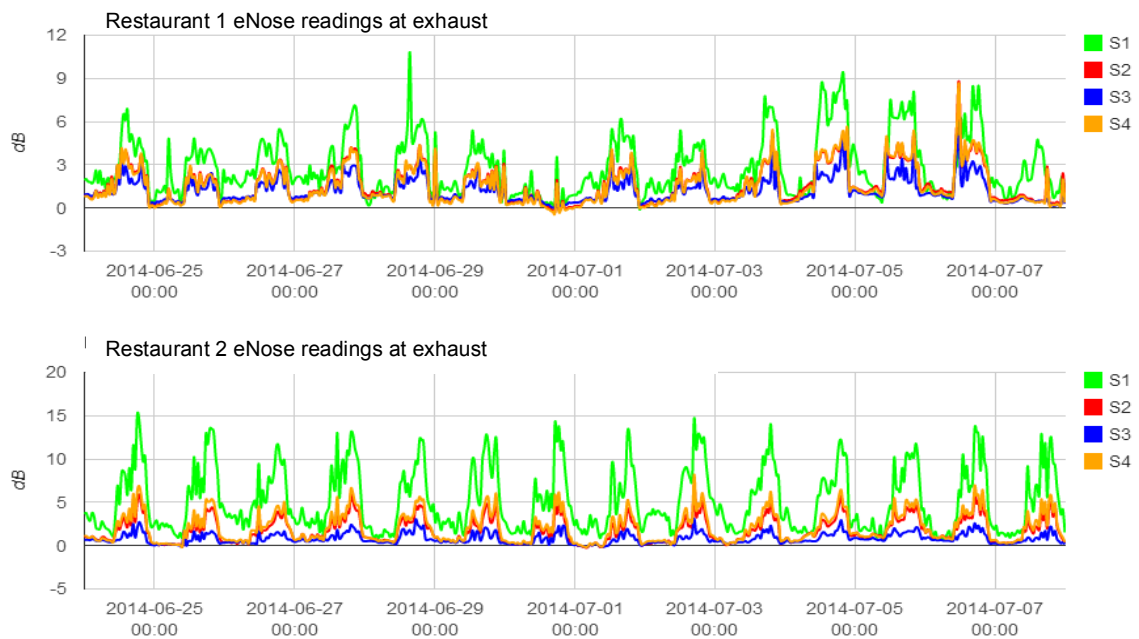
Figure 1: Raw eNose data of the exhausts of restaurants 1 and 2 show a good relationship with the operating times of the restaurants being monitored.
