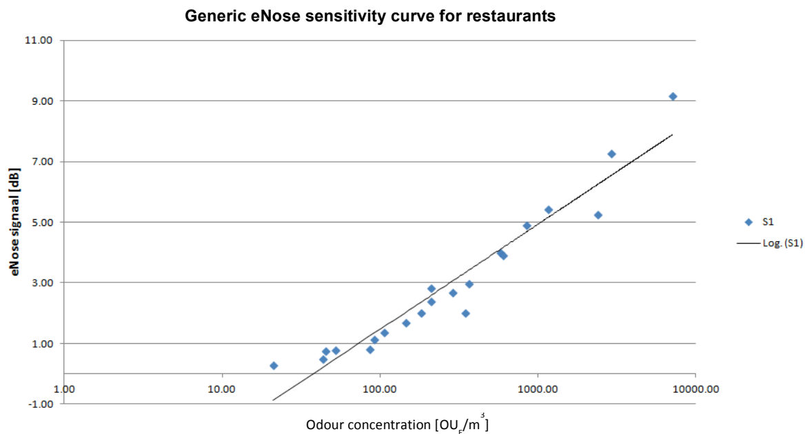
Figure 4: Generic eNose “restaurants-sensitivity-curve”
